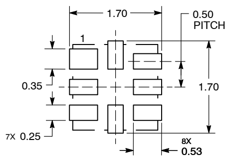
DETAIL A OPTIONAL CONSTRUCTION
