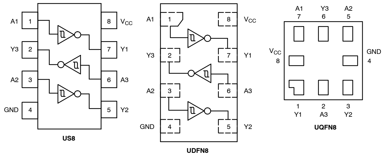
Figure 2. Pinout
