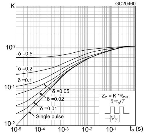
Figure 2. Thermal impedance
