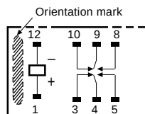
Terminal arrangement/ Internal connections (Top view)
