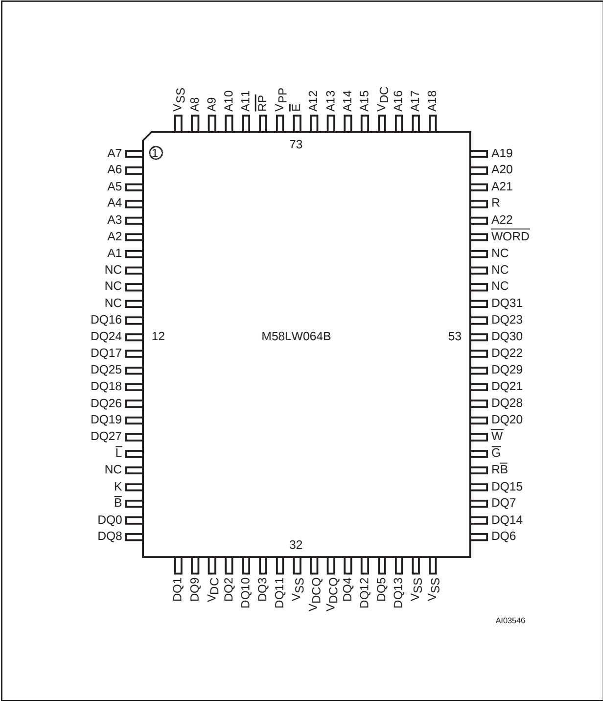
Figure 5. PQFP Connections
