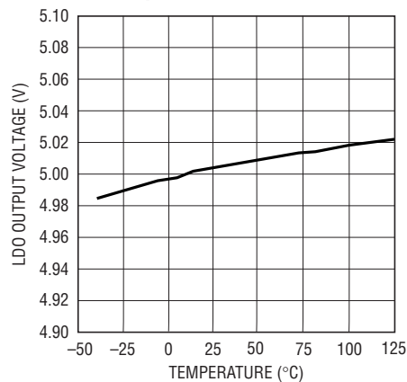
5V LDO Output Voltage vs Temperature
