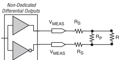
Figure 1-8. Output Delay Timing Report Setup for Differential Outputs with Three External Resistor
