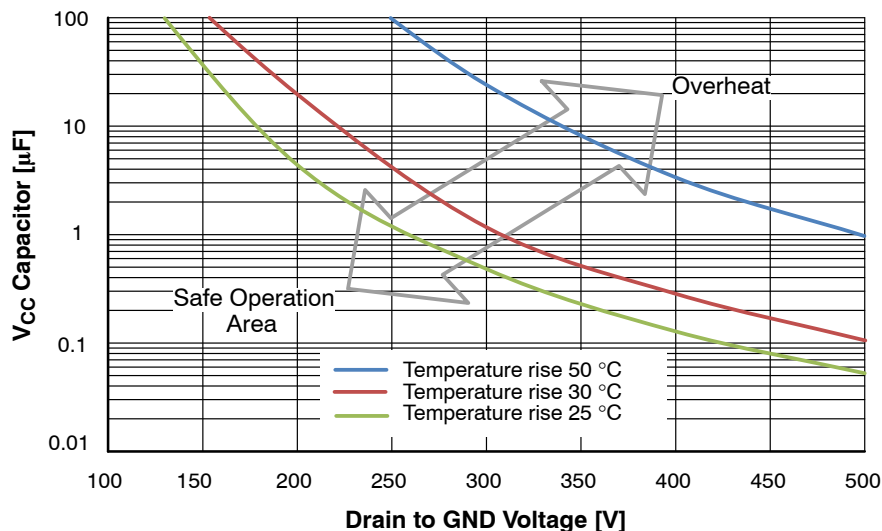
Figure 32. SOA V_{\text{CC}} Capacitor Selection
