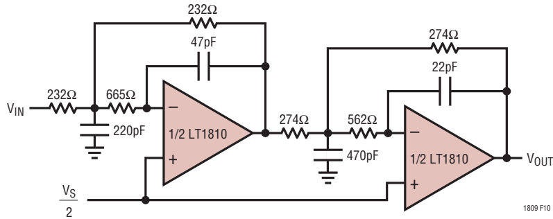
Figure 10. Single 3V Supply, 4MHz, 4th Order Butterworth Filter
