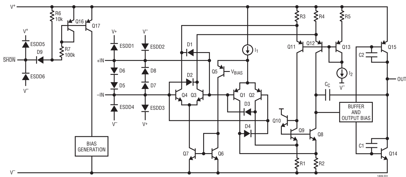
Figure 1. LT1809 Simplified Schematic Diagram
