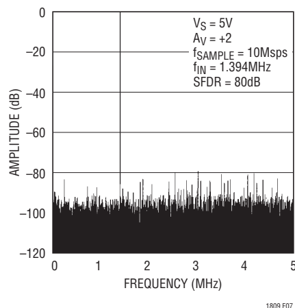
Figure 7. 4096 Point FFT Response
