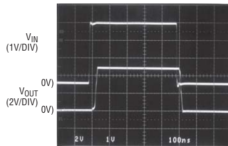
Output Overdriven Recovery
