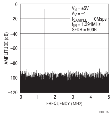
Figure 5. 4096 Point FFT Response
