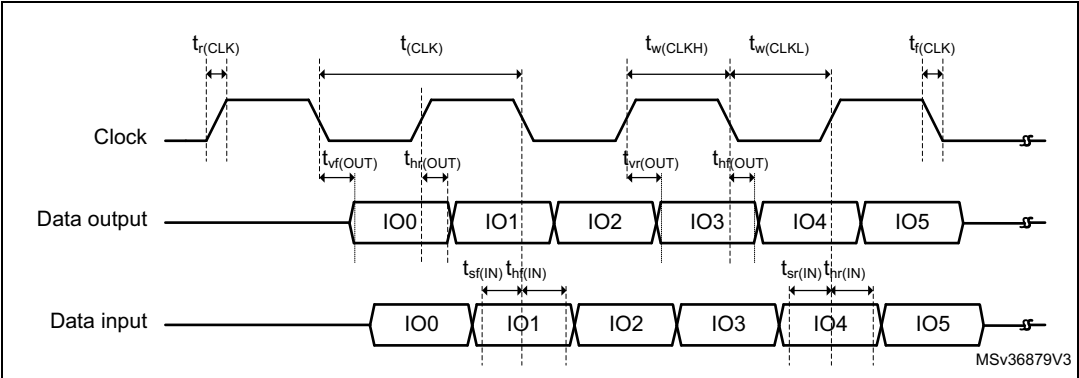
Figure 68. OCTOSPI timing diagram - DDR mode
