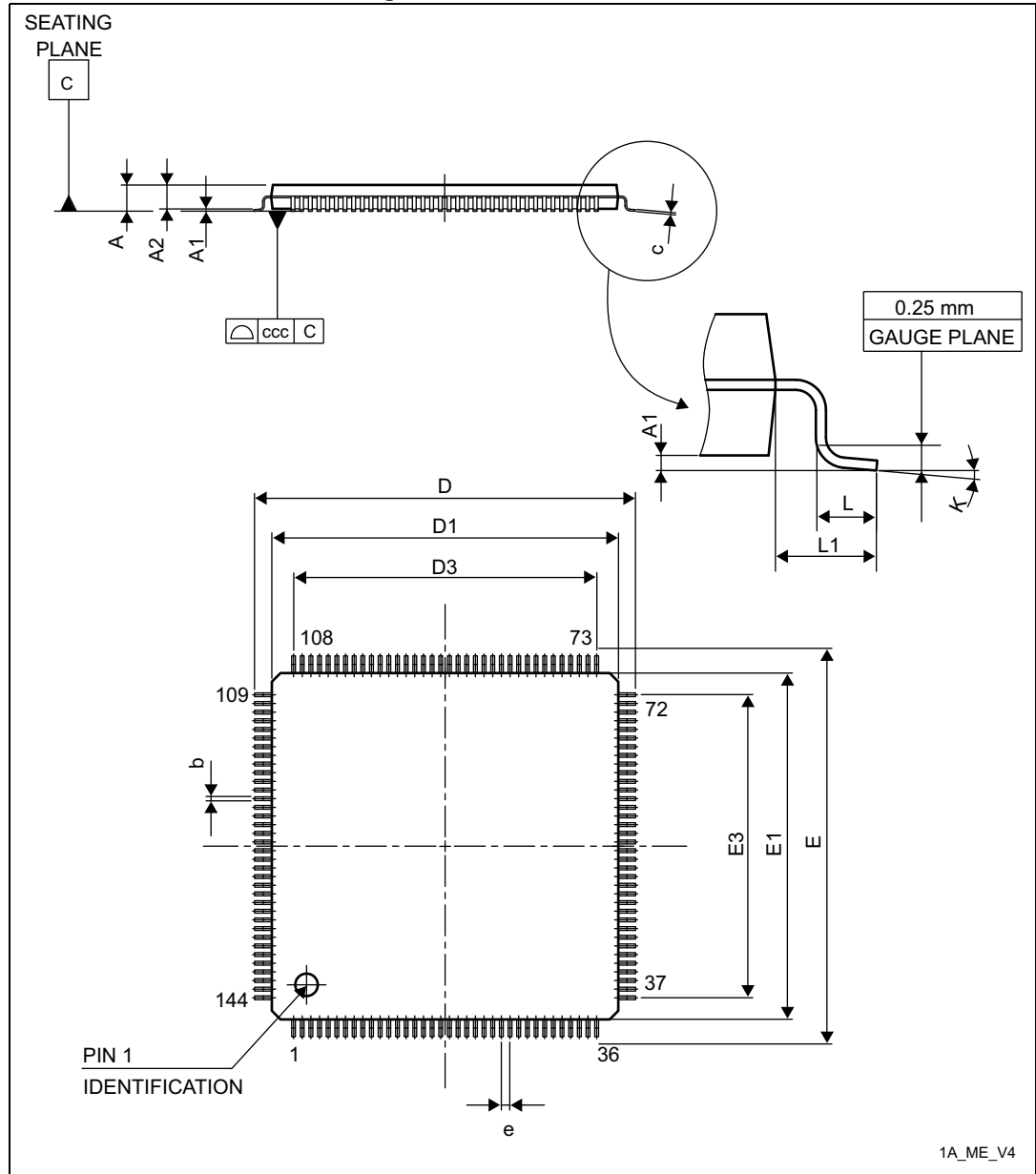
Figure 94. LQFP144 outline
