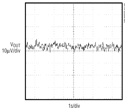
MAX6023EBT12 0.1Hz TO 10Hz OUTPUT NOISE
