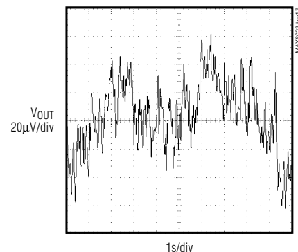
MAX6023EBT50 0.1Hz TO 10Hz OUTPUT NOISE
