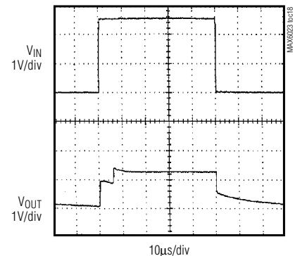
MAX6023EBT12 TURN-ON TRANSIENT
