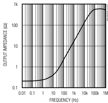
MAX6023EBT12 OUTPUT IMPEDANCE vs. FREQUENCY
