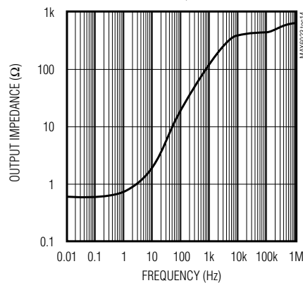
MAX6023EBT50 OUTPUT IMPEDANCE vs. FREQUENCY
