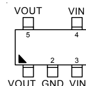
SOT-23-5 (L-Type)
