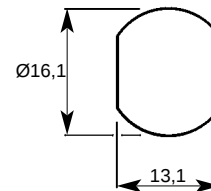
FIXING HOLE SIZE
