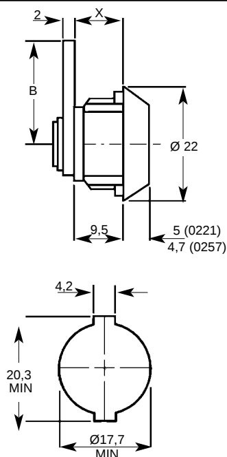
FIXING HOLE SIZE
