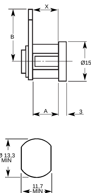
FIXING HOLE SIZE
