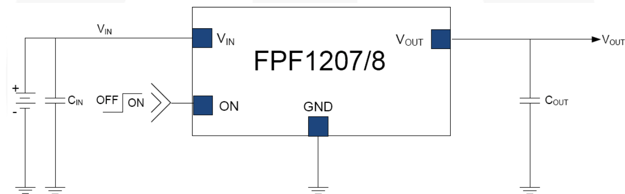
Figure 26. Typical Application
