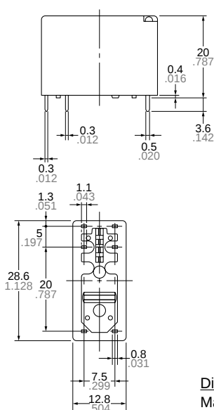
2 Form A
