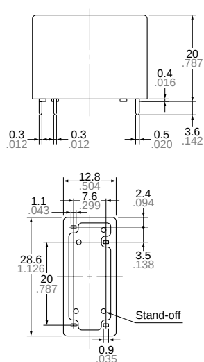
1 Form A
