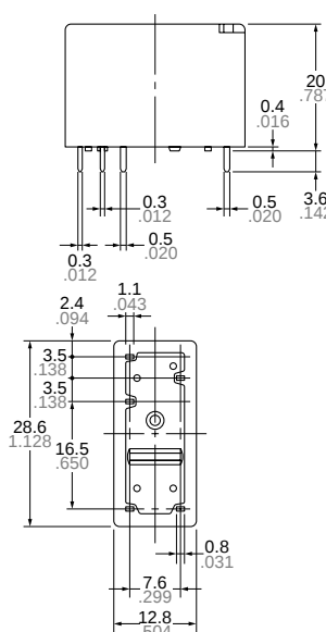
1 Form C
