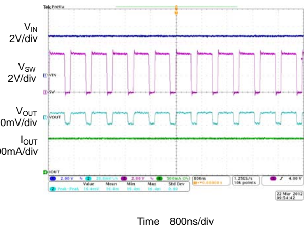
Figure 17. V_{OUT} Ripple ( V_{IN}=5V , V_{OUT}=3.3V , I_{OUT}=1000mA )
