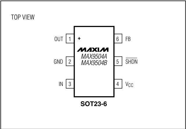
Pin Configurations (continued)
