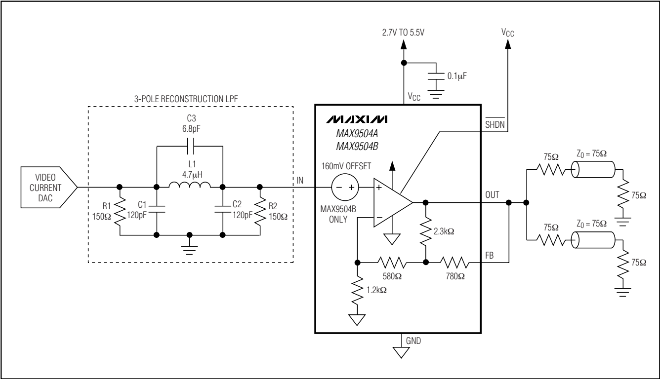
Typical Operating Circuit
