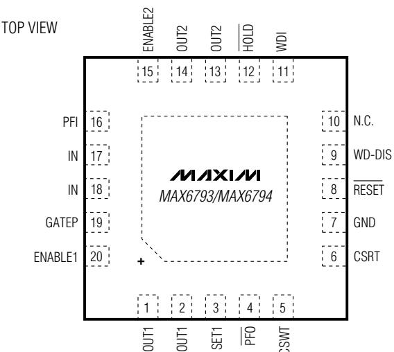
THIN QFN 5mm x 5mm
