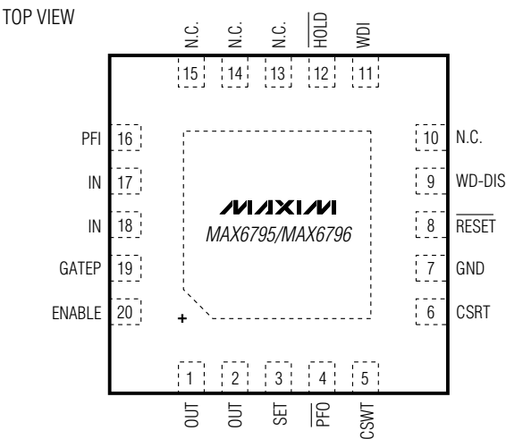
THIN QFN 5mm x 5mm
