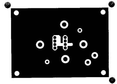
FIGURE 1C. BOTTOM LAYOUT
