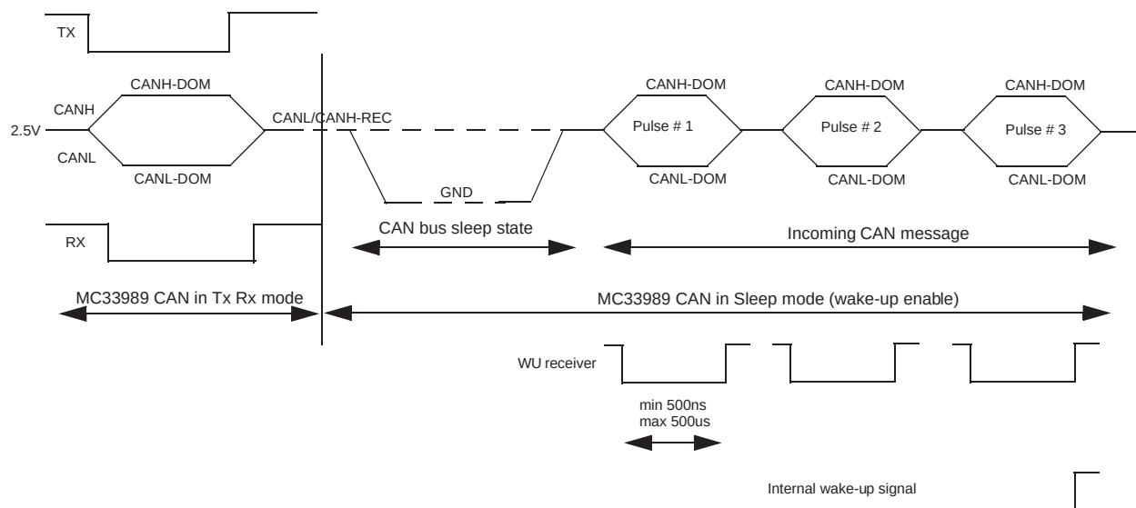
Figure 40. Pattern Wake-Up
