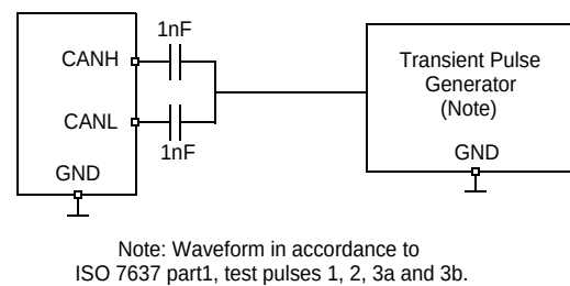
Figure 6. Transient Test Pulses for CANH/CANL
