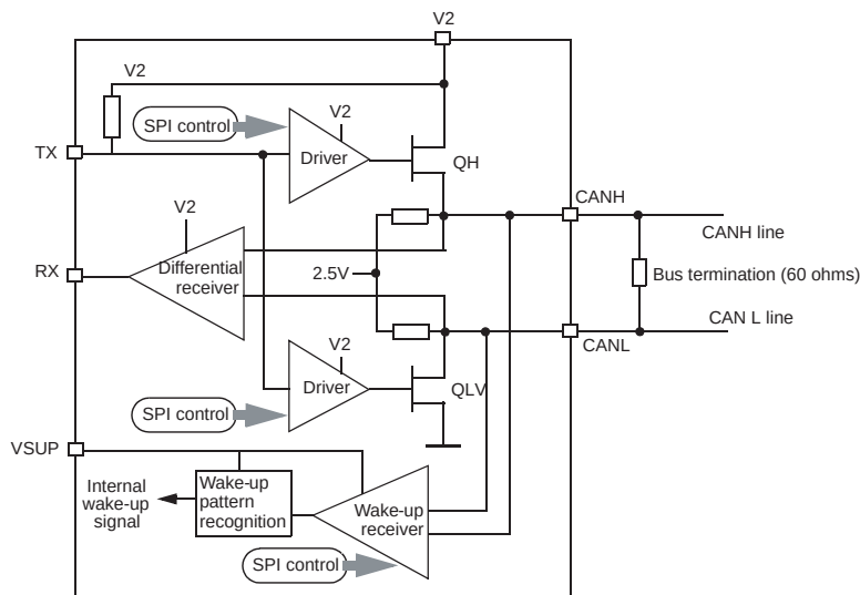
Figure 34. 33989 CAN Interface
