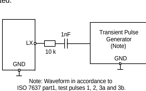
Figure 5. Transient Test Pulse for L0:L3 Inputs
