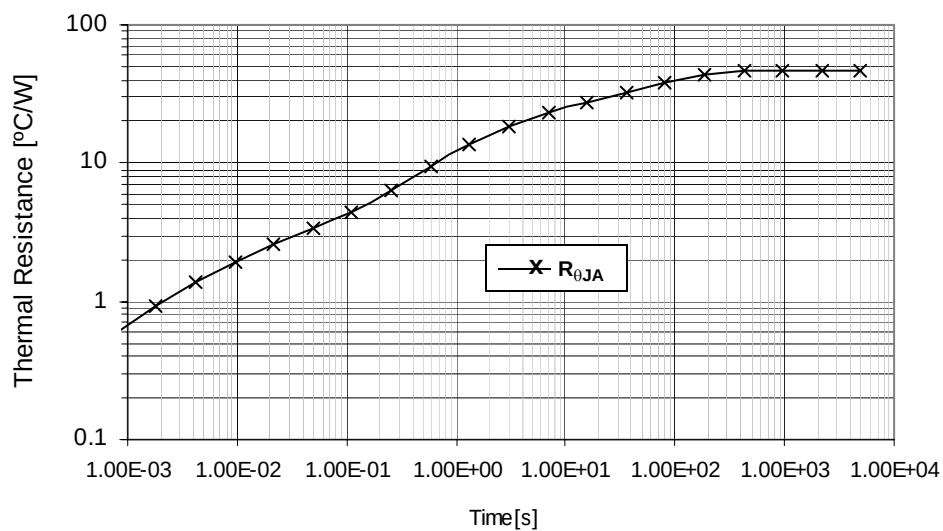
Figure 65. Transient Thermal Resistance R_{\theta JA} 1 W Step response, Device on Thermal Test Board Area A = 600 (mm²)
