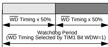
Figure 17. Window Watchdog
