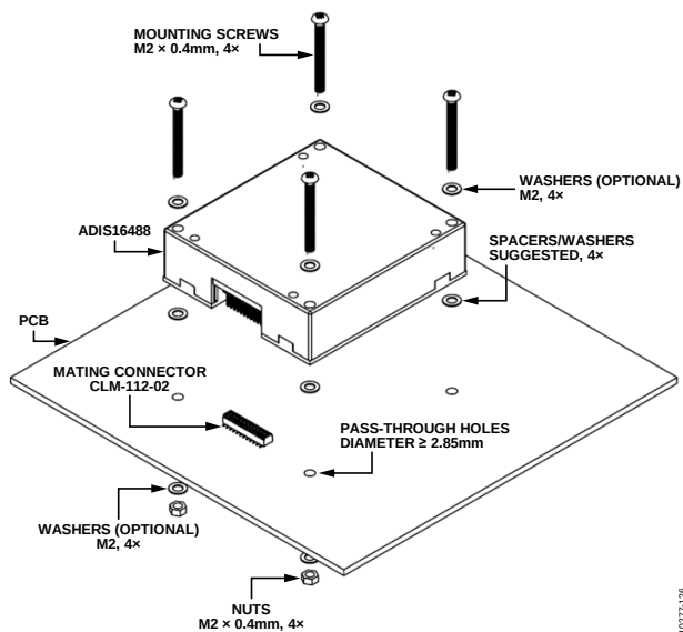
Figure 26. Mounting Example
