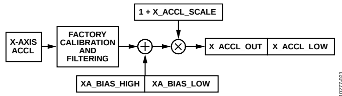
Figure 23. User Calibration Signal Path, Gyroscopes
