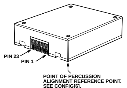
Figure 24. Point of Percussion Reference Point
