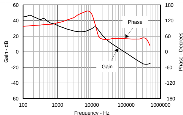
Figure 12. Loop Response, I_{\text{OUT}} = 0.25\text{ A}
