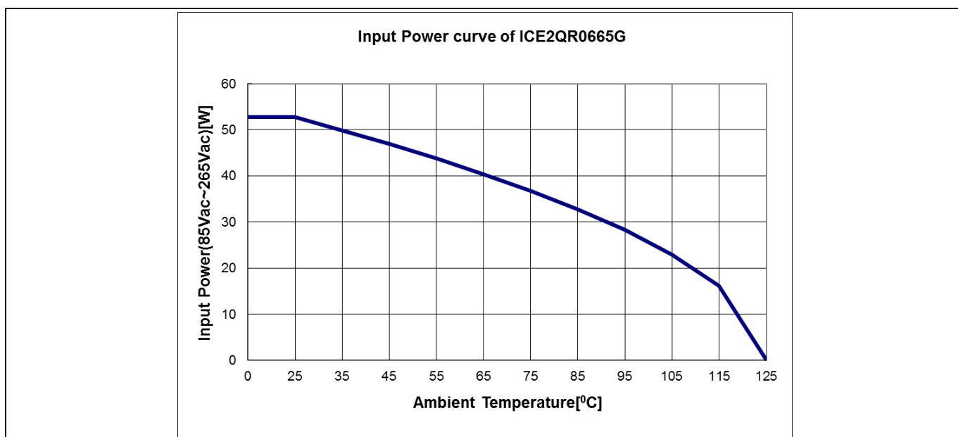
Figure 13 Input power curve V_{in}=85\sim 265 V_{AC} ; P_{in}=f(T_a)
