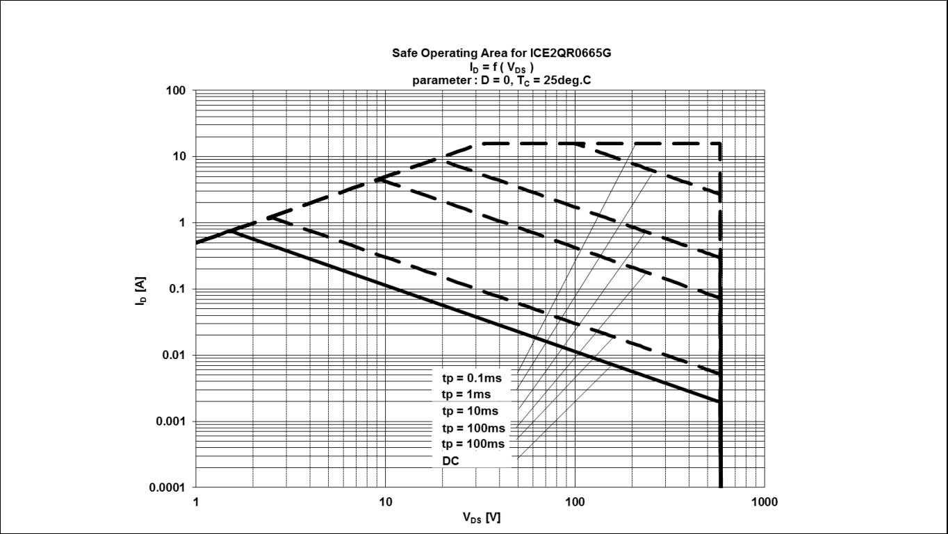
Figure 10 Safe Operating Area (SOA) curve for ICE2QR0665G
