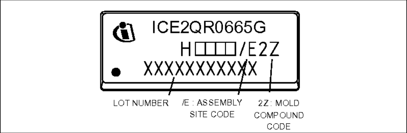
Figure 16 Marking for ICE2QR0665G
