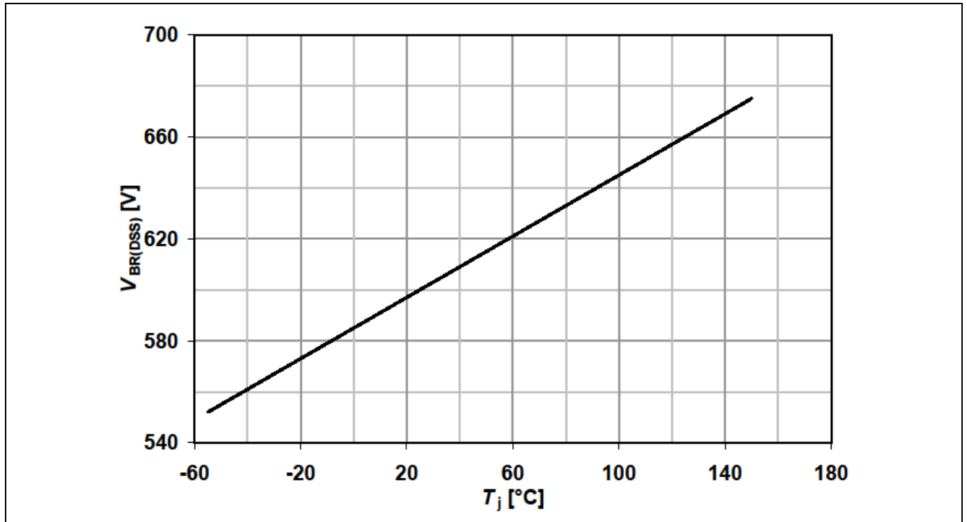
Figure 12 Drain-source breakdown voltage; V_{BR(DSS)} = f(T_j) , I_D = 0.25\text{mA}
