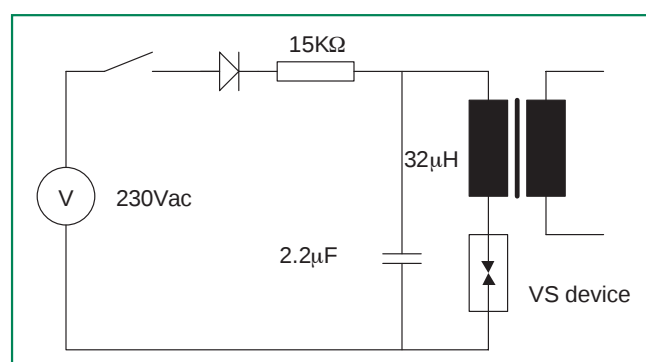
Fig 2. Recommended Life Test Circuit
