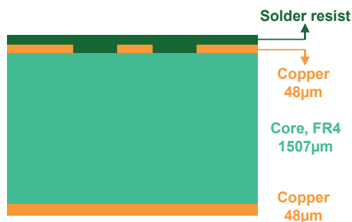
Figure 14. PCB stack-up recommendations
