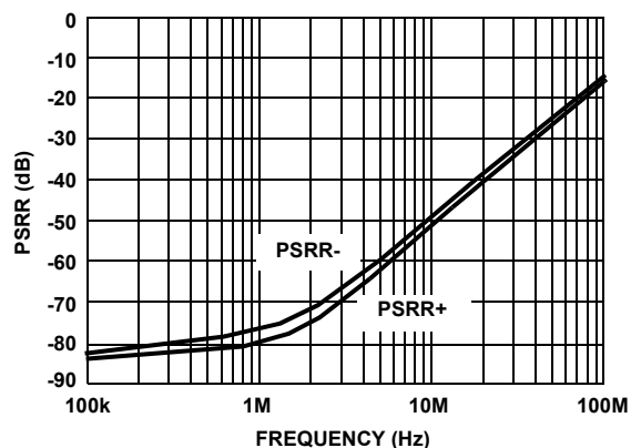
FIGURE 5. POWER SUPPLY REJECTION RATIO vs FREQUENCY
