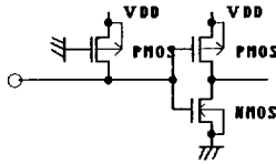
Input Terminal Structure
