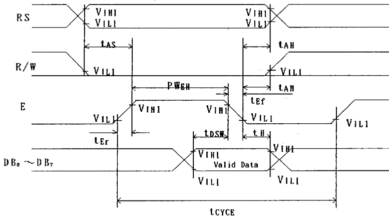
fig. 1 The timing characteristics of the bus write operating sequence. (Write from MPU to NJU6427)
