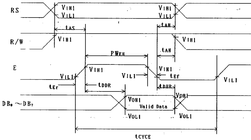
fig. 2 The timing characteristics of the bus read operating sequence. (Read from NJU6427 to MPU)
