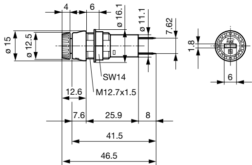
Variants Fingergrip 3101.0115 and 3101.0315
