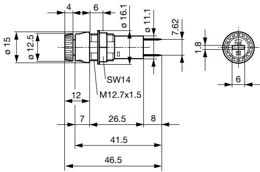
Variants Fingergrip 3101.0015 and 3101.0215
