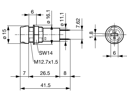
Variants 3101.0010 and 3101.0210
