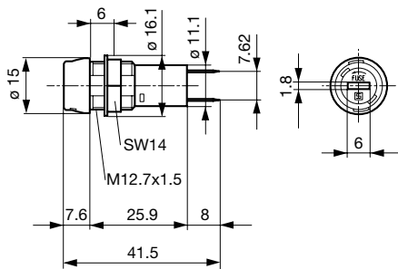
Variants 3101.0110 and 3101.0310
