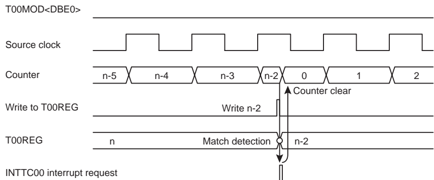
Figure 14-3 Operation When T00REG and the Up Counter Have the Same Value
