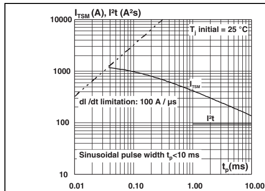
Figure 7. Non repetitive surge peak on-state current and corresponding values of I^2t
