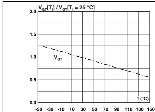
Figure 9. Relative variation of gate trigger voltage versus junction temperature (typical values)
