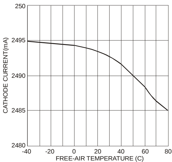
Reference Voltage vs. Free-Air Temperature
