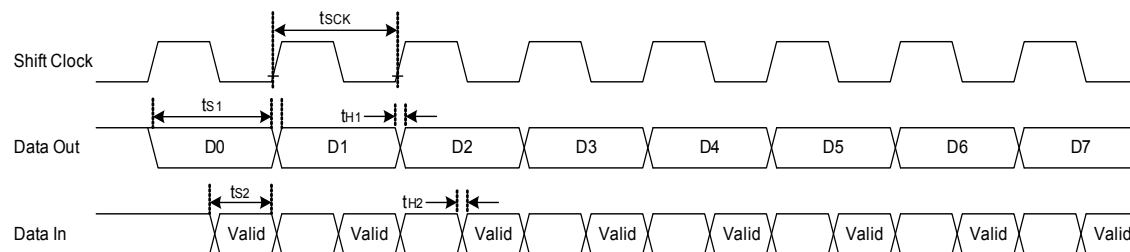
Figure 7.5 Timing Waveform for the UART Module
