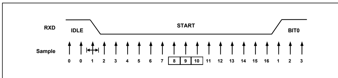
Figure 11.39 Start Bit Sampling
