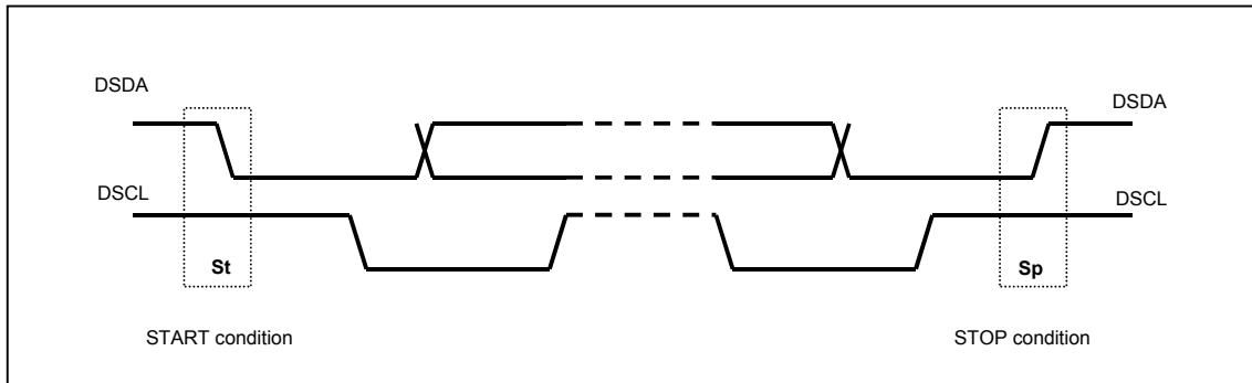
Figure 14.5 Start and Stop Condition
