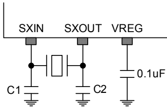
Figure 7.10 Crystal Oscillator
