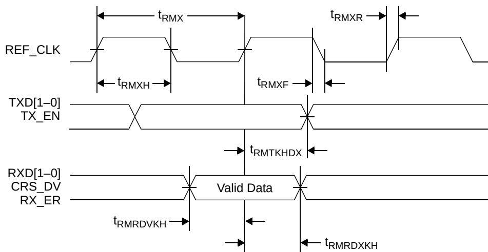
Figure 28. RMII Transmit and Receive AC Timing
