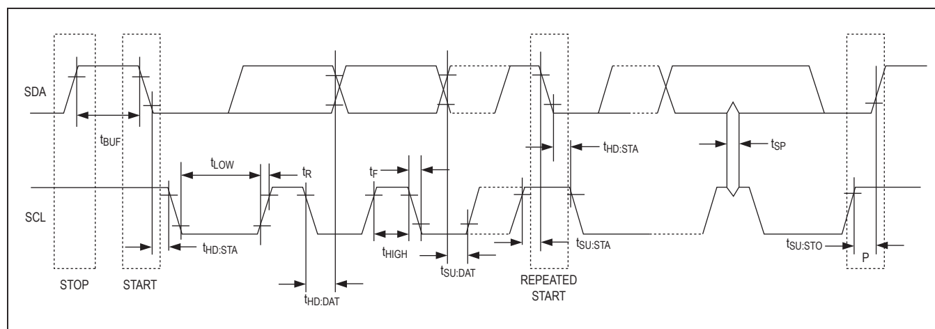
Figure 1. I²C Serial Interface Timing Diagram
