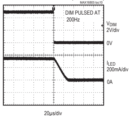
LED CURRENT FALL TIME (EXPANDED)
