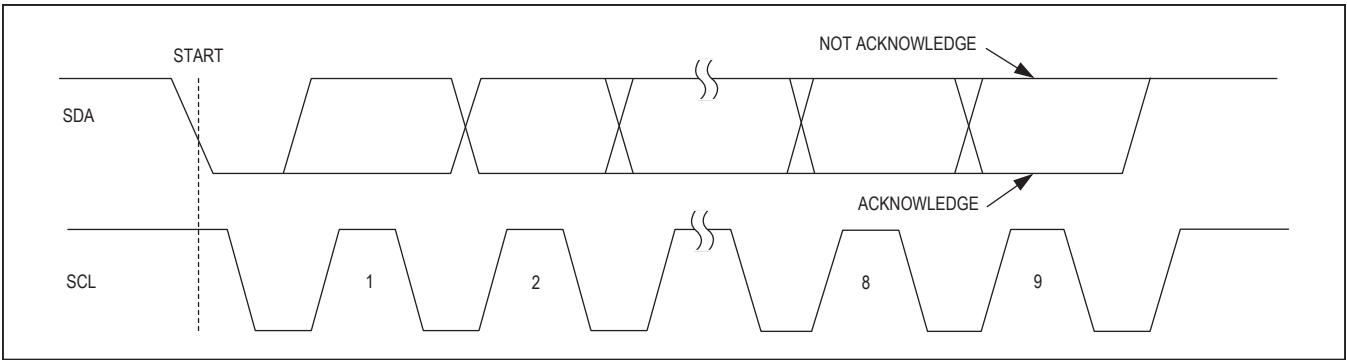
Figure 5. Acknowledge
