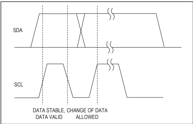
Figure 4. Bit Transfer
