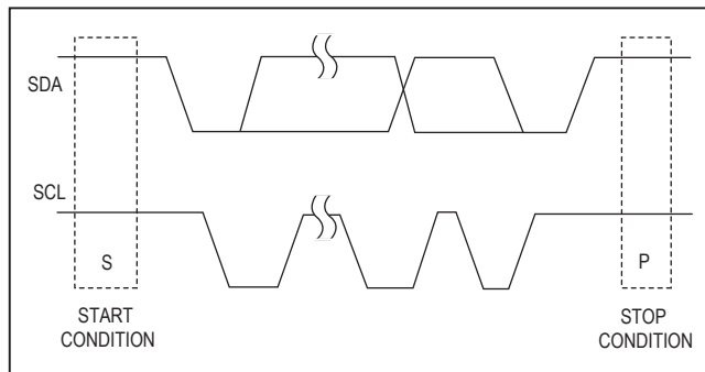
Figure 3. I 2 C Communication Start and Stop Conditions
