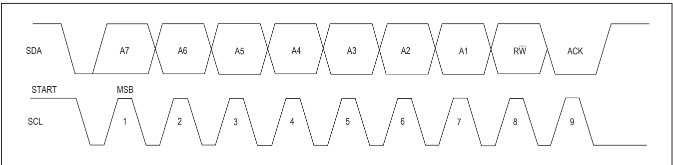
Figure 6. Slave Address
