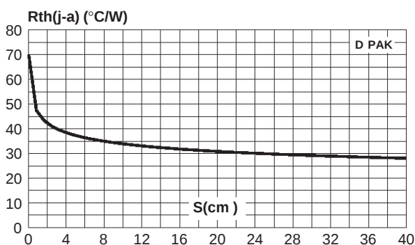
Fig. 10: D PAK Thermal resistance junction to ambient versus copper surface under tab (printed circuit board FR4, copper thickness: 35\text{ }\mu\text{m} ).
