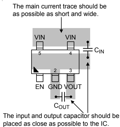
Figure 3. PCB Layout Guide for SOT-23-5 Package
