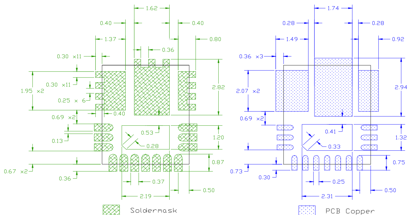
Figure 32: Solder Resist
