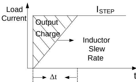
Figure 28: Charge Requirement during Load Step
