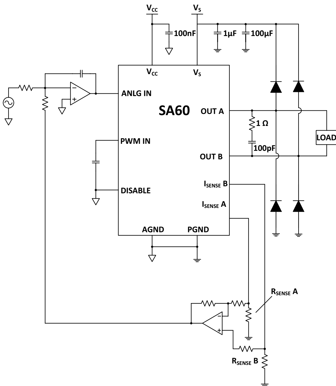
Figure 1: Typical Connection
