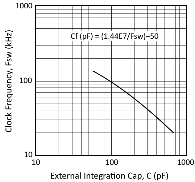
Figure 11: PWM Frequency vs. External Integration Capacitor
