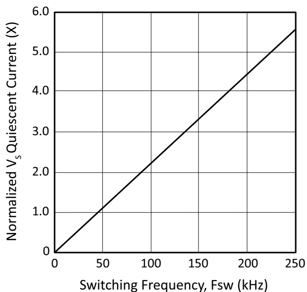
Figure 9: V_s Quiescent vs. Switch Frequency
