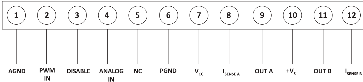
Figure 2: External Connections
