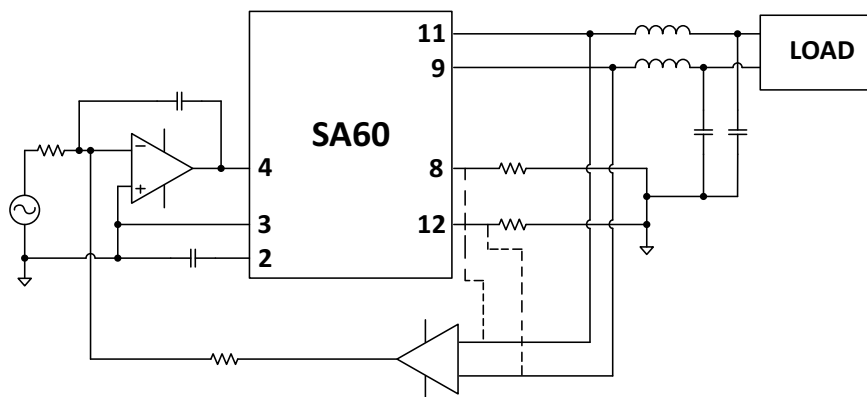
Figure 12: Typical Application
