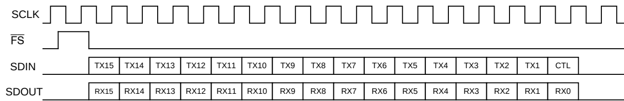
Data Frame with earlyl Frame Sync
