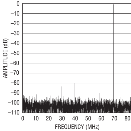
8192 Point FFT, f IN = 70MHz, -1dB, 2V Range, LVDS Mode
