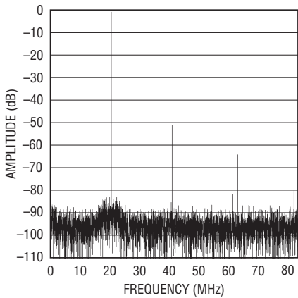
8192 Point FFT, f IN = 1GHz, -1dB, 1V Range, LVDS Mode
