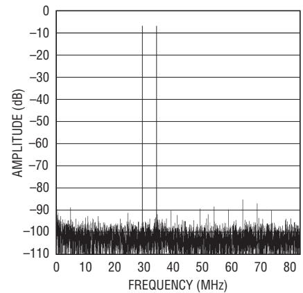
8192 Point 2-Tone FFT, f IN = 135MHz and 140MHz, -1dB, 2V Range, LVDS Mode
