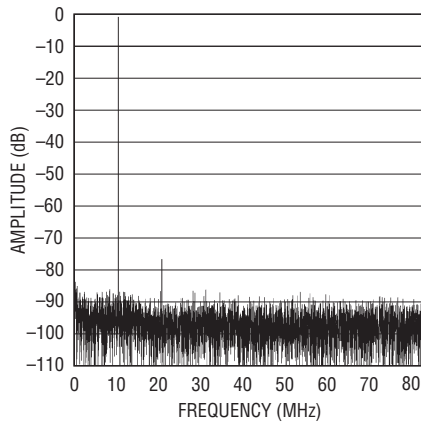
8192 Point FFT, f IN = 500MHz, -1dB, 1V Range, LVDS Mode
