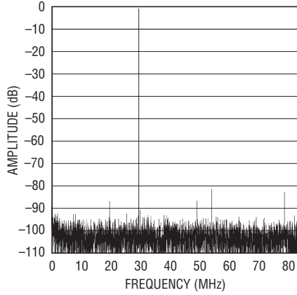
8192 Point FFT, f IN = 140MHz, -1dB, 2V Range, LVDS Mode
