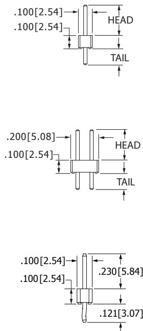
RETENTION LEAD MOUNTING (EXAMPLE P/N: AMC36SAAR)
