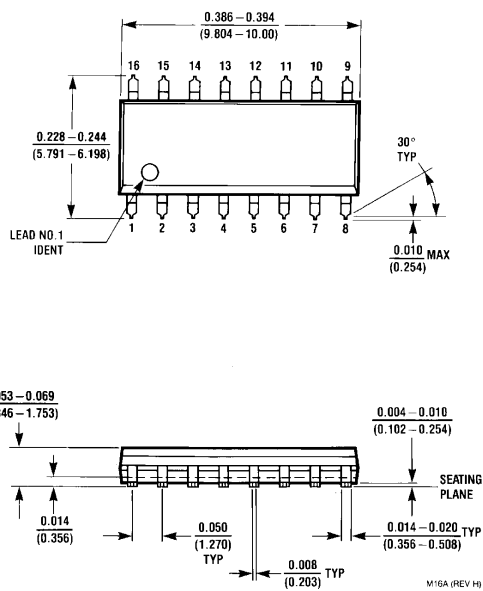
16-Lead Small Outline Integrated Circuit (SOIC), JEDEC MS-012, 0.150 Narrow Package Number M16A
