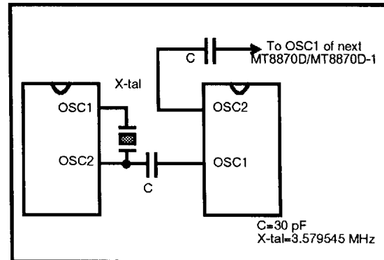
Figure 7 - Oscillator Connection
