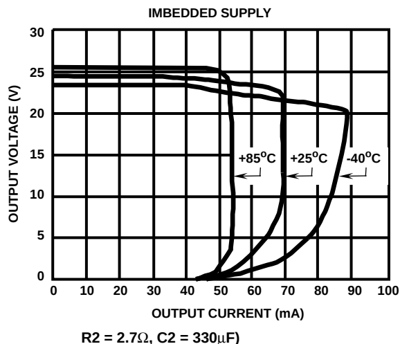
FIGURE 13. OUTPUT CURRENT vs TEMPERATURE ( R1 = 150\Omega , R2 = 2.7\Omega , C2 = 330\mu F )
