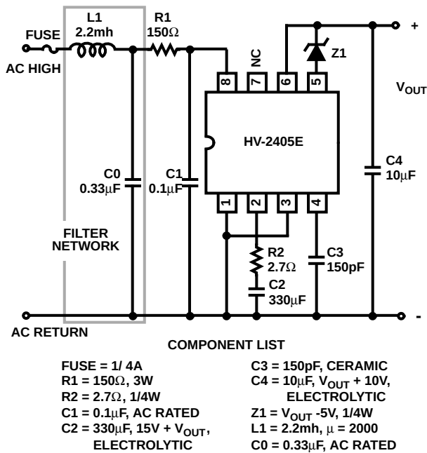
FIGURE 8. IMBEDDED SUPPLY WITH EMI FILTER ( I_{OUT} \leq 30mA )
