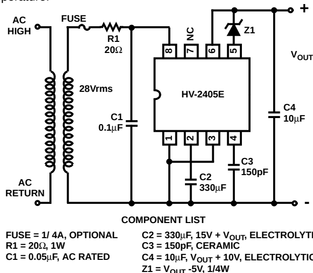
FIGURE 14. LOW INPUT VOLTAGE SUPPLY
