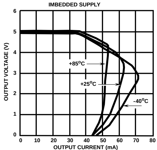
FIGURE 12. OUTPUT CURRENT vs TEMPERATURE ( R1 = 150\Omega ,
