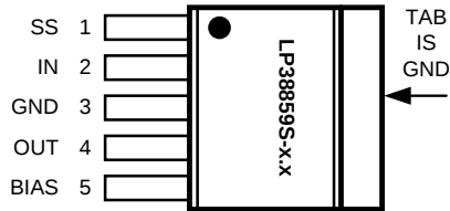
Figure 1. 5-Lead DDPAK/TO-263, Top View See KTT Package
