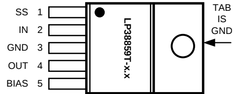
Figure 2. 5-Lead TO-220, Top View See NDH005D Package
