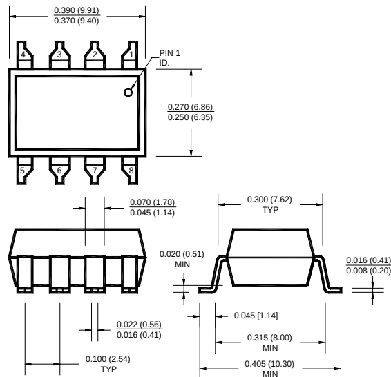
Package Dimensions (Surface Mount)
