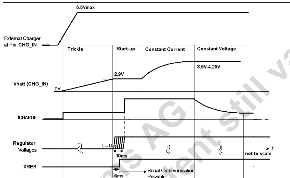
Figure 24 Charger States
