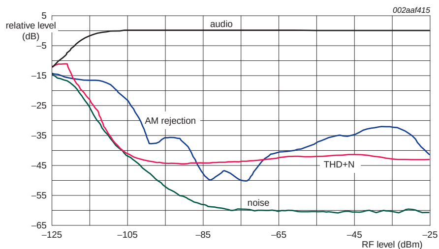
Fig 9. Relative level of audio, AM rejection, THD+N and noise versus RF level ( T_{amb} = -40\text{ °C} )
