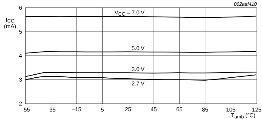
Fig 4. Supply current versus ambient temperature
