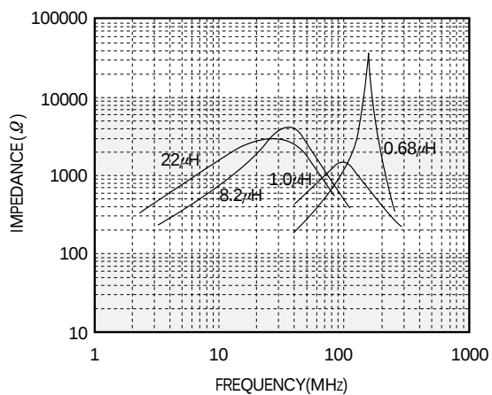
■IMPEDANCE CHARACTERISTICS
