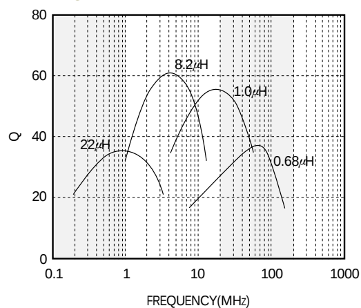
■Q CHARACTERISTICS
