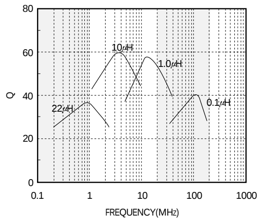
■Q CHARACTERISTICS
