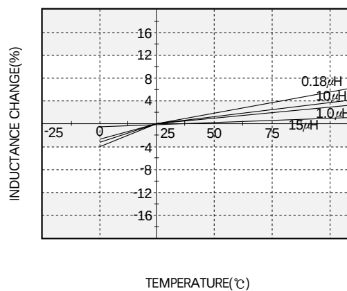
■TEMPERATURE CHARACTERISTICS
