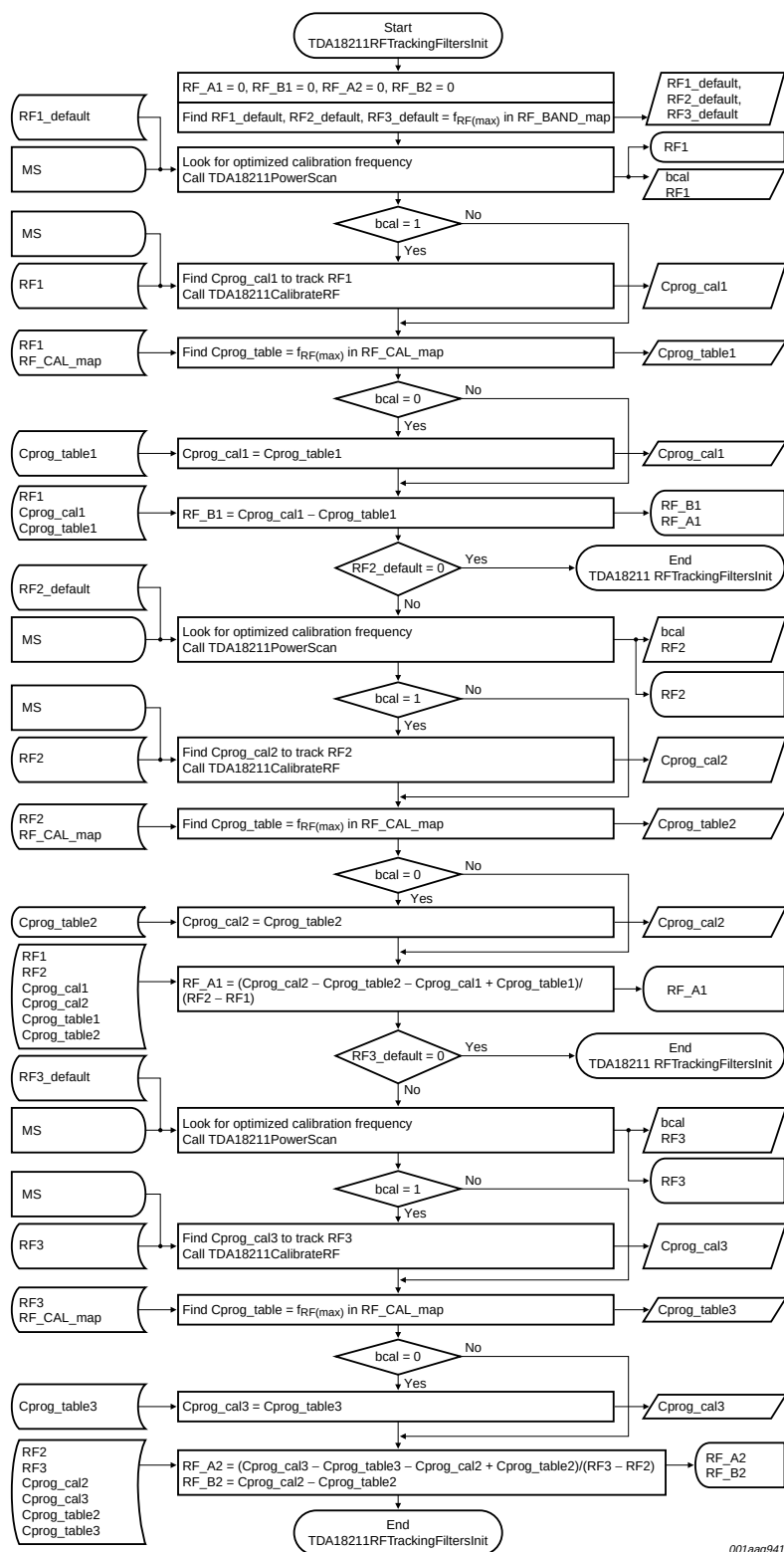
Fig 11. Flowchart TDA18211RFTrackingFiltersInit
