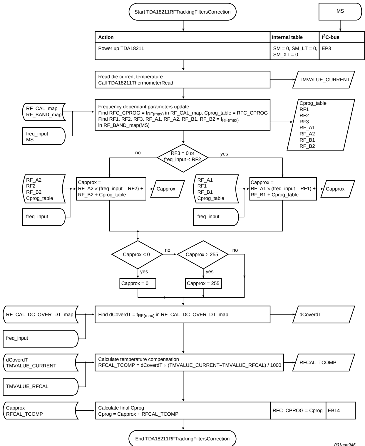
Fig 16. Flowchart TDA18211RFTrackingFiltersCorrection
