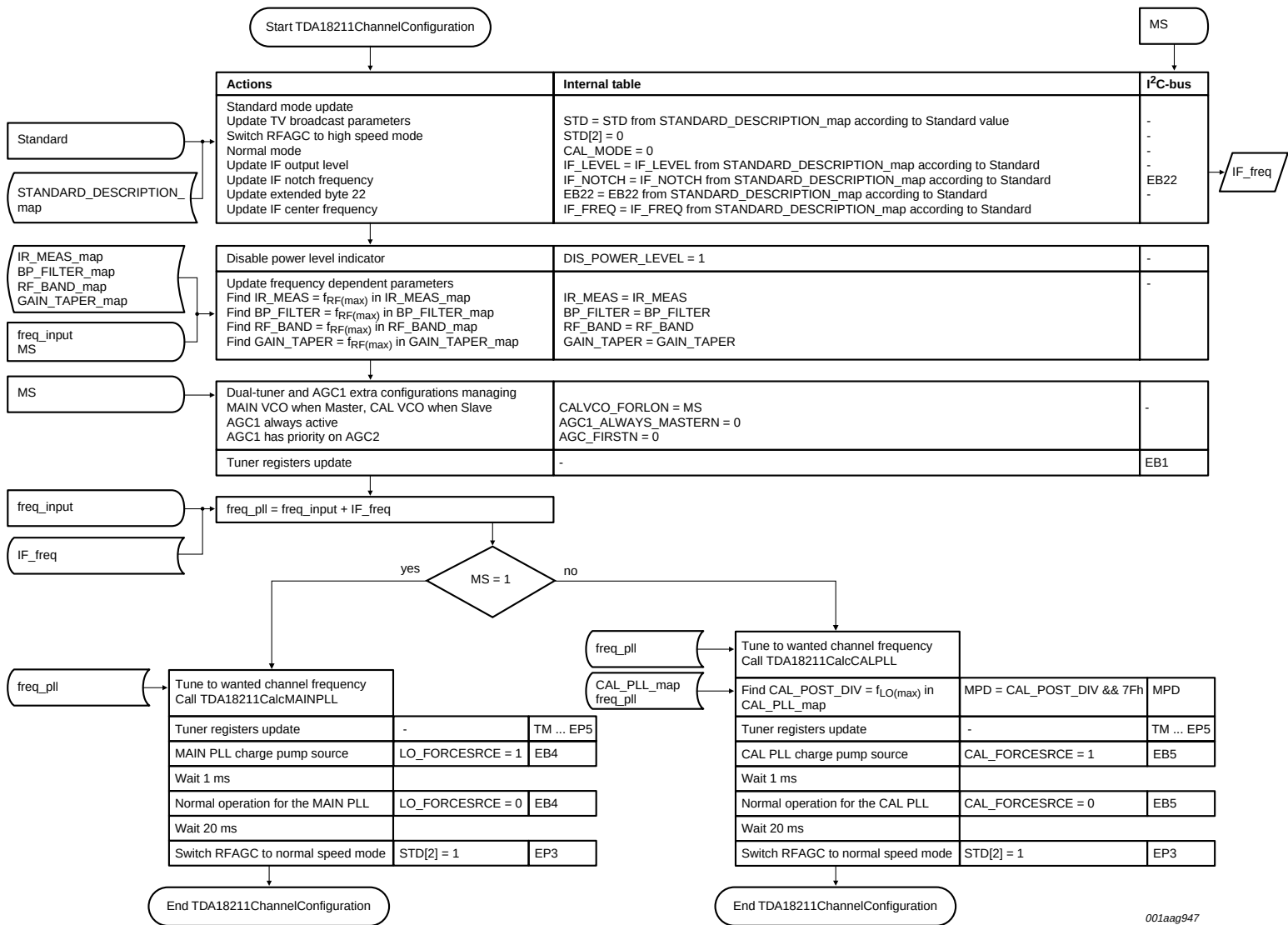
Fig 17. Flowchart TDA18211ChannelConfiguration
