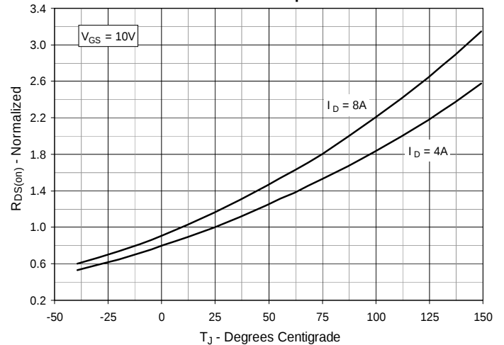
Fig. 4. R_{DS(on)} Normalized to I_D = 4\text{A} Value vs. Junction Temperature
